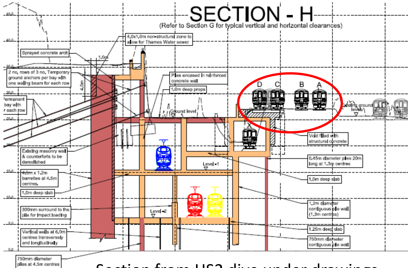
Section from HS2 dive under drawings for Park Village East
